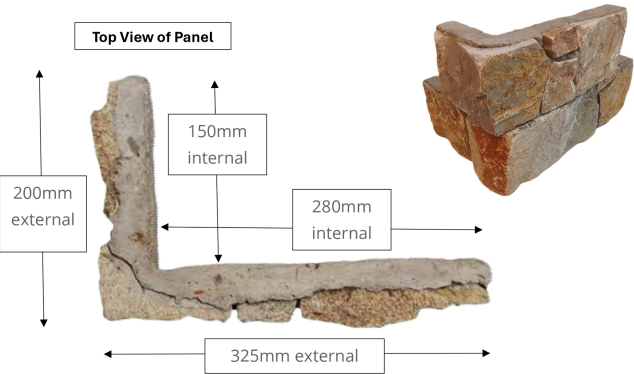
Pre-Formed Corner Panels - 200mm high x (280mm + 150mm returns)
