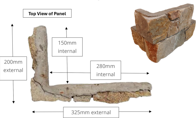
Pre-Formed Corner Panels - 200mm high x (280mm + 150mm returns)
