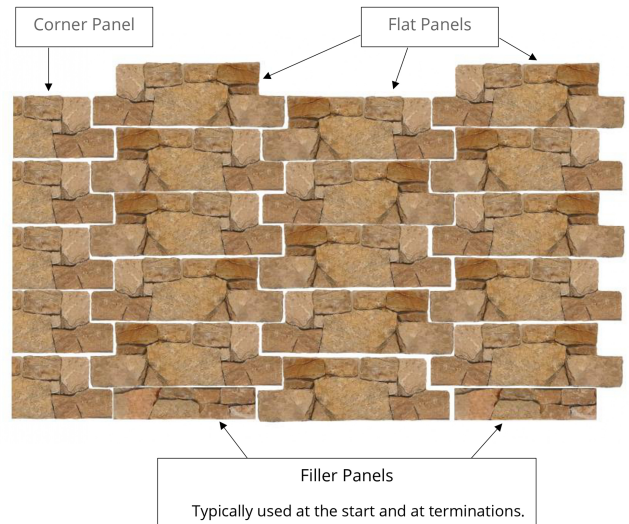
Typical Panel Configuration
