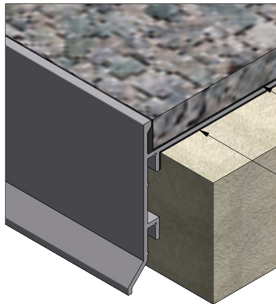
Typical installation detail
