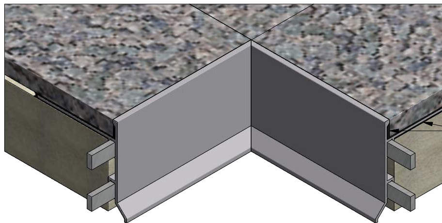
Typical installation detail
